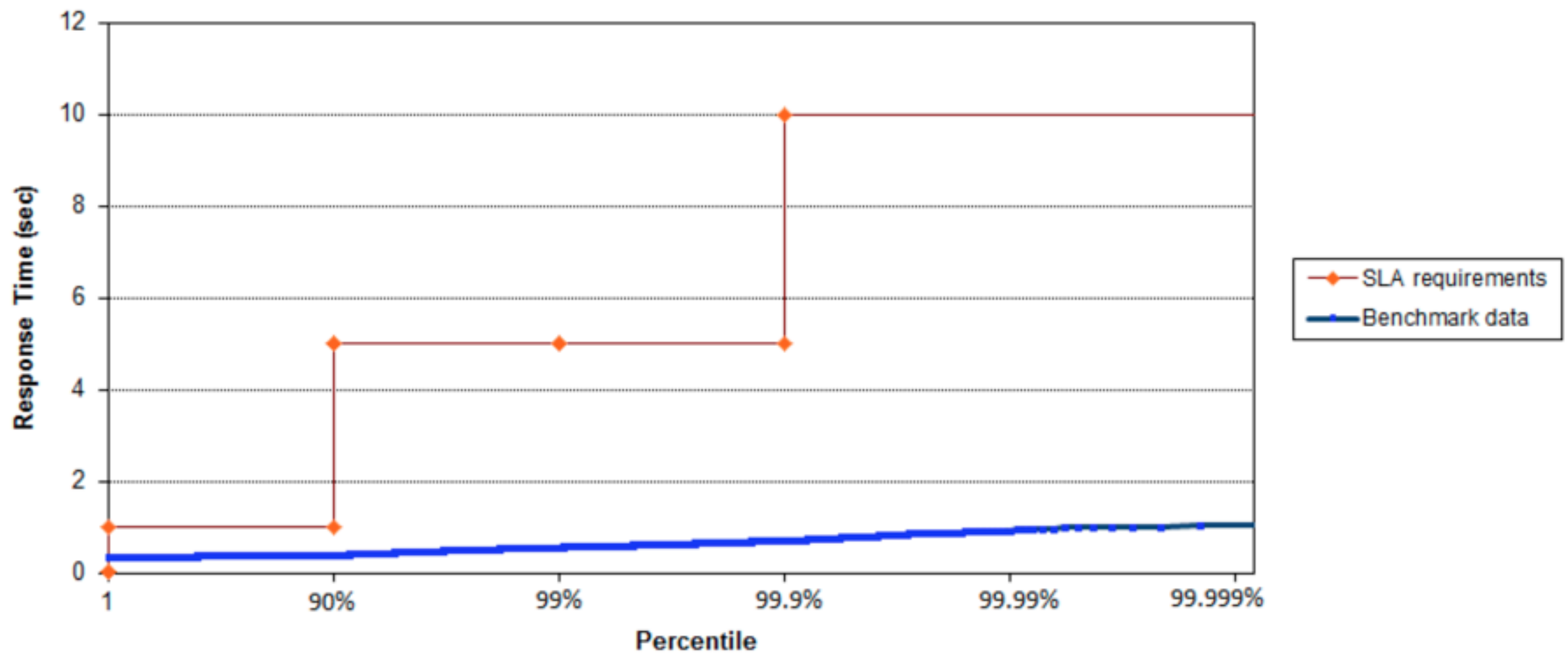
Zing @ 800 users with 50 GB heap
